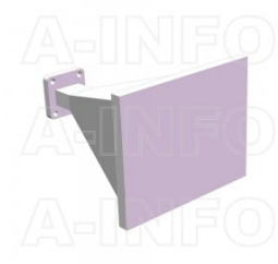
LB-42-20-ASPO Standard Gain Horn Antenna 18-26.5GHz 20dB Gain Rectangular Waveguide Interface
